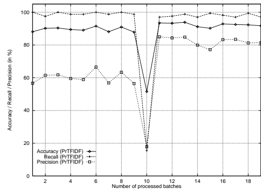
Figure 6: Performance measures accuracy, recall, and precision for the Adaptive Size approach in combination with PrTFIDF for scenario A.
